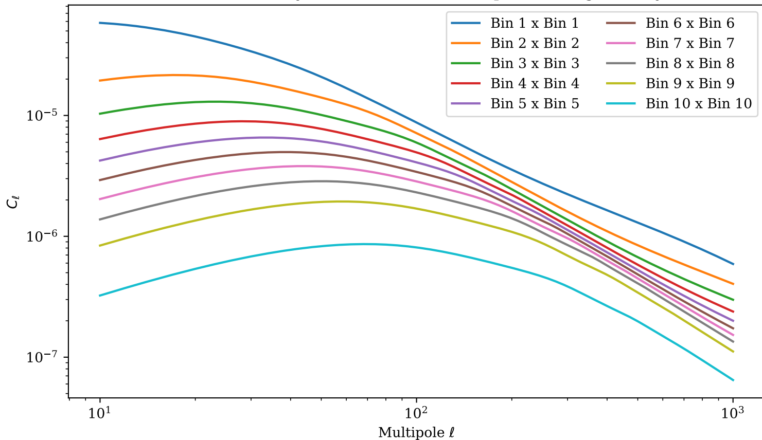
LSST Y10 Galaxy Auto-Correlation Comparison (Signal Only)
