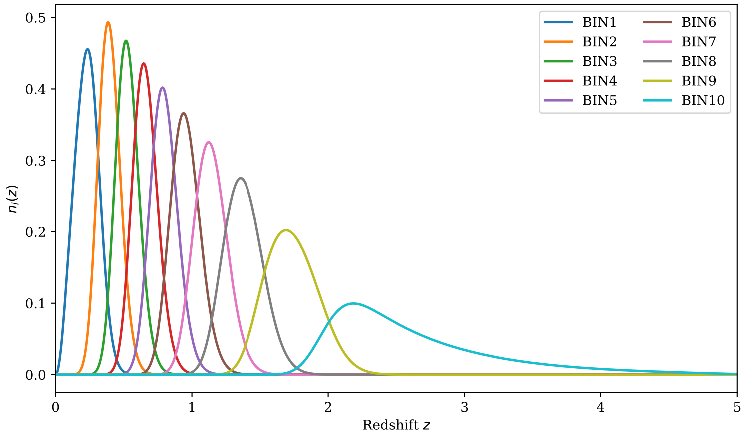
LSST Y10 Galaxy Tomographic Redshift Distributions
