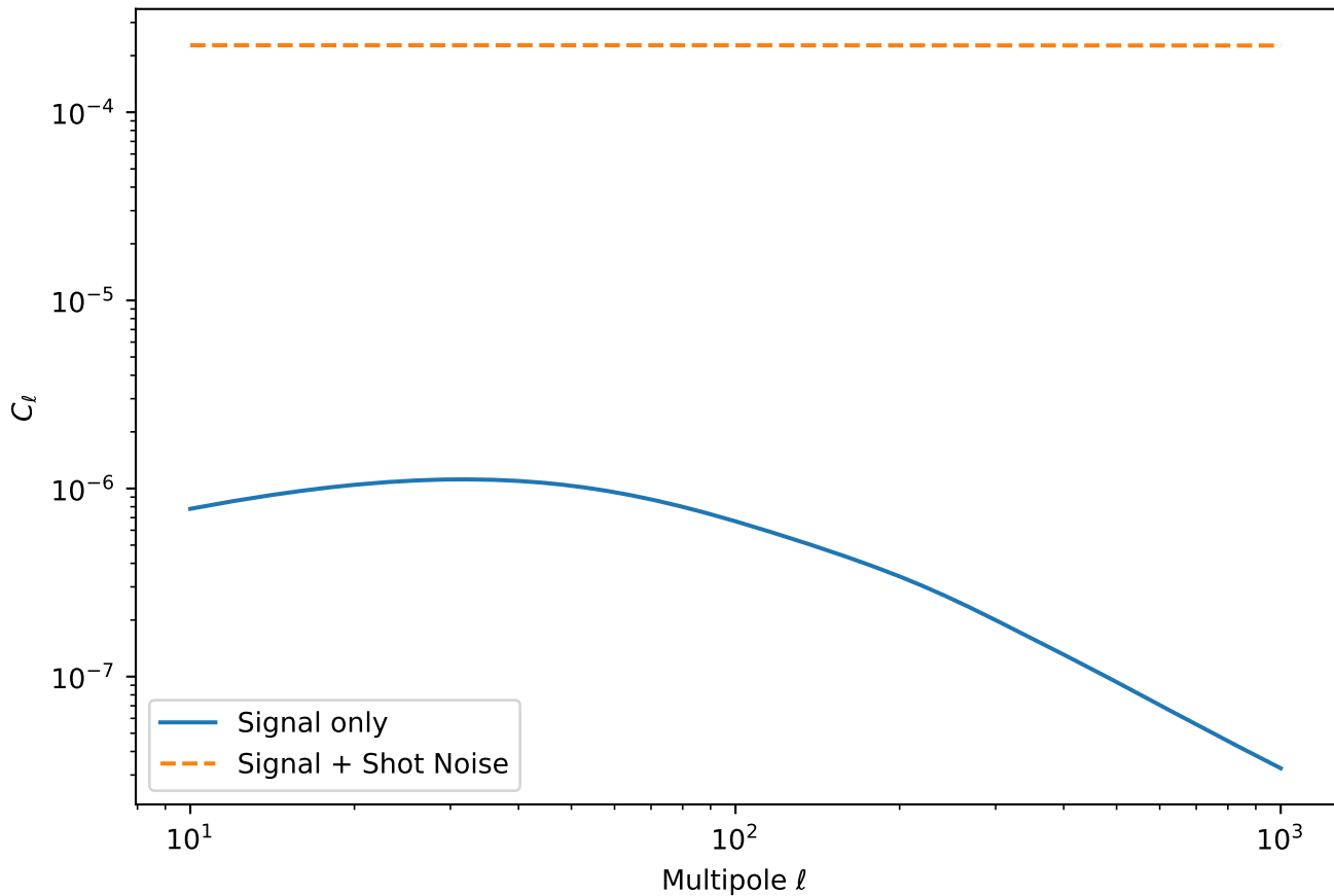
FRB Auto-Correlation Angular Power Spectrum (Deep Survey) for Magnetars
