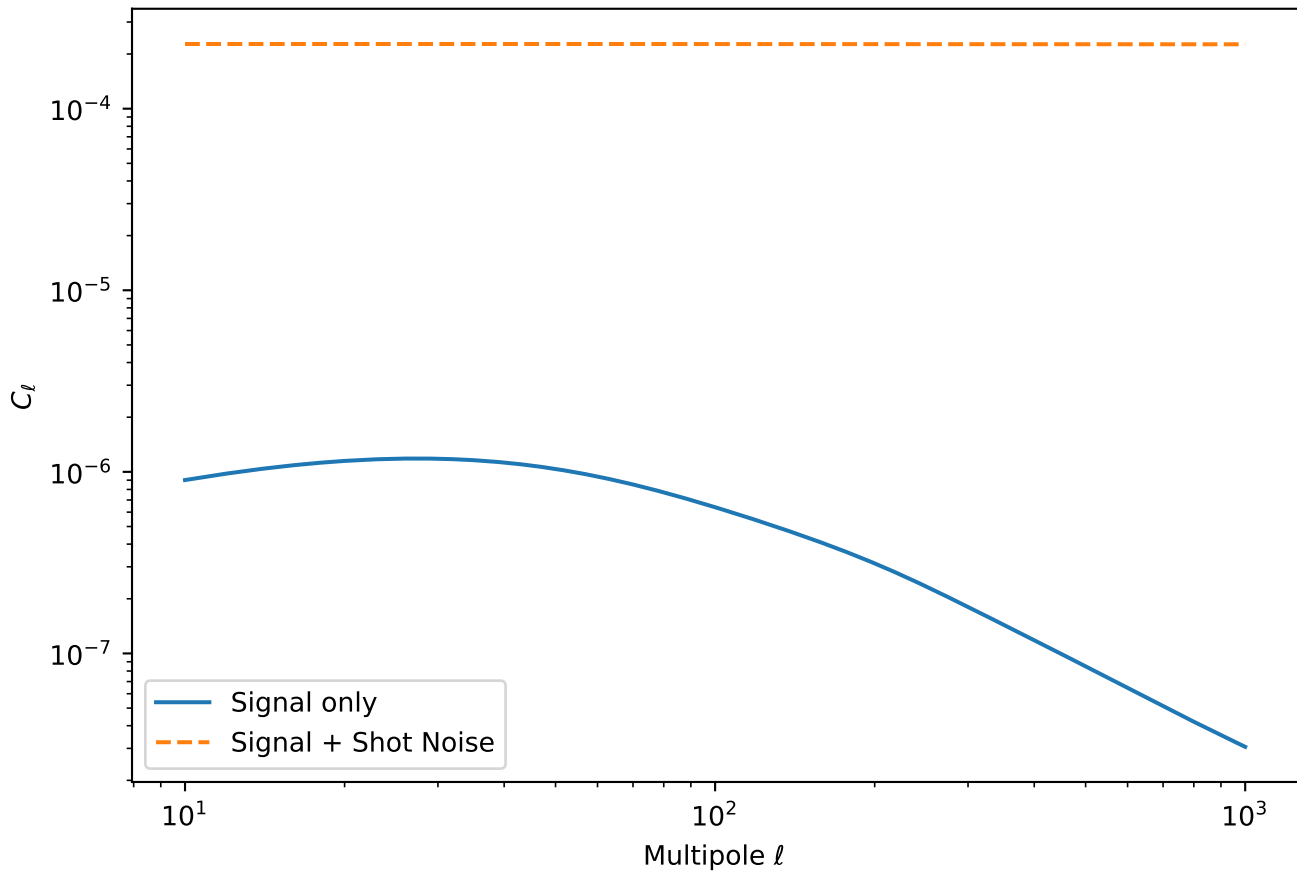
FRB Auto-Correlation Angular Power Spectrum (Deep Survey) for Neutron Star
