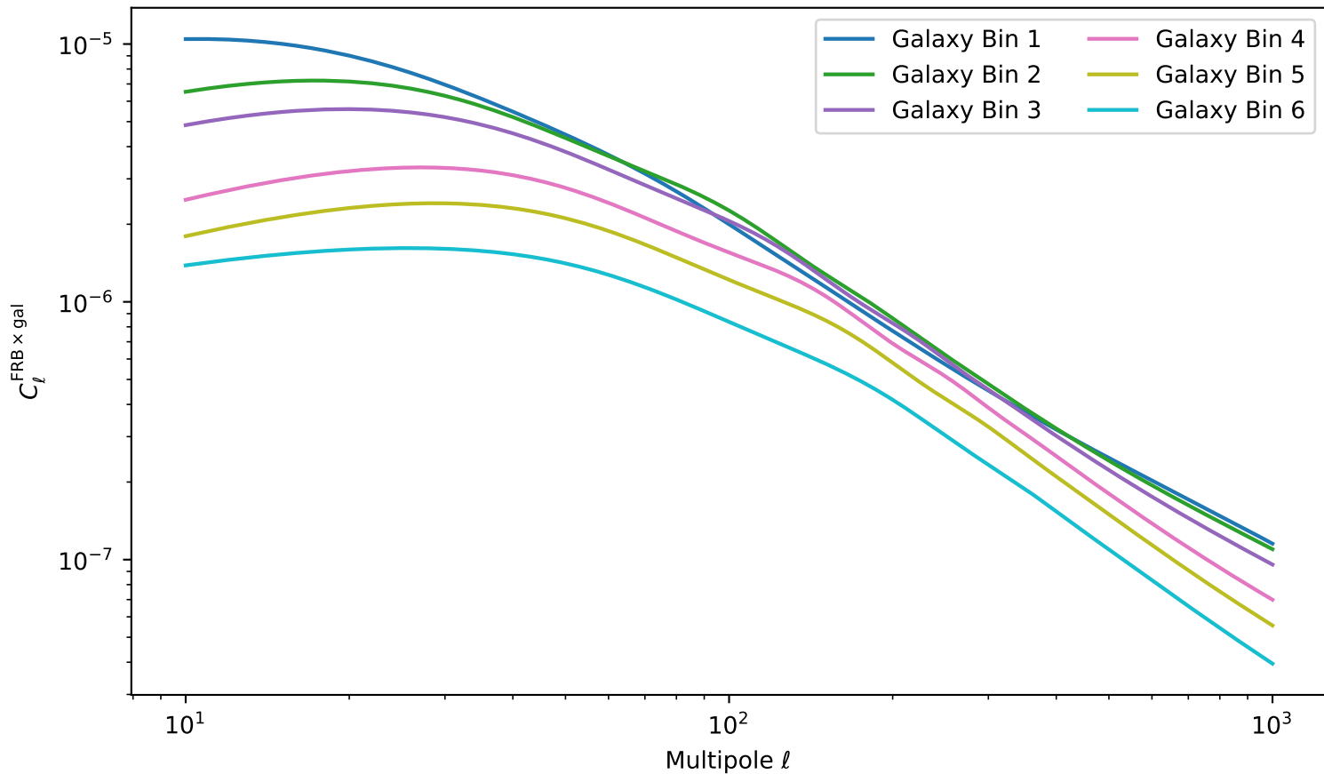
FRB×Galaxy — All Bins (Neutron Stars, Shallow Survey)
