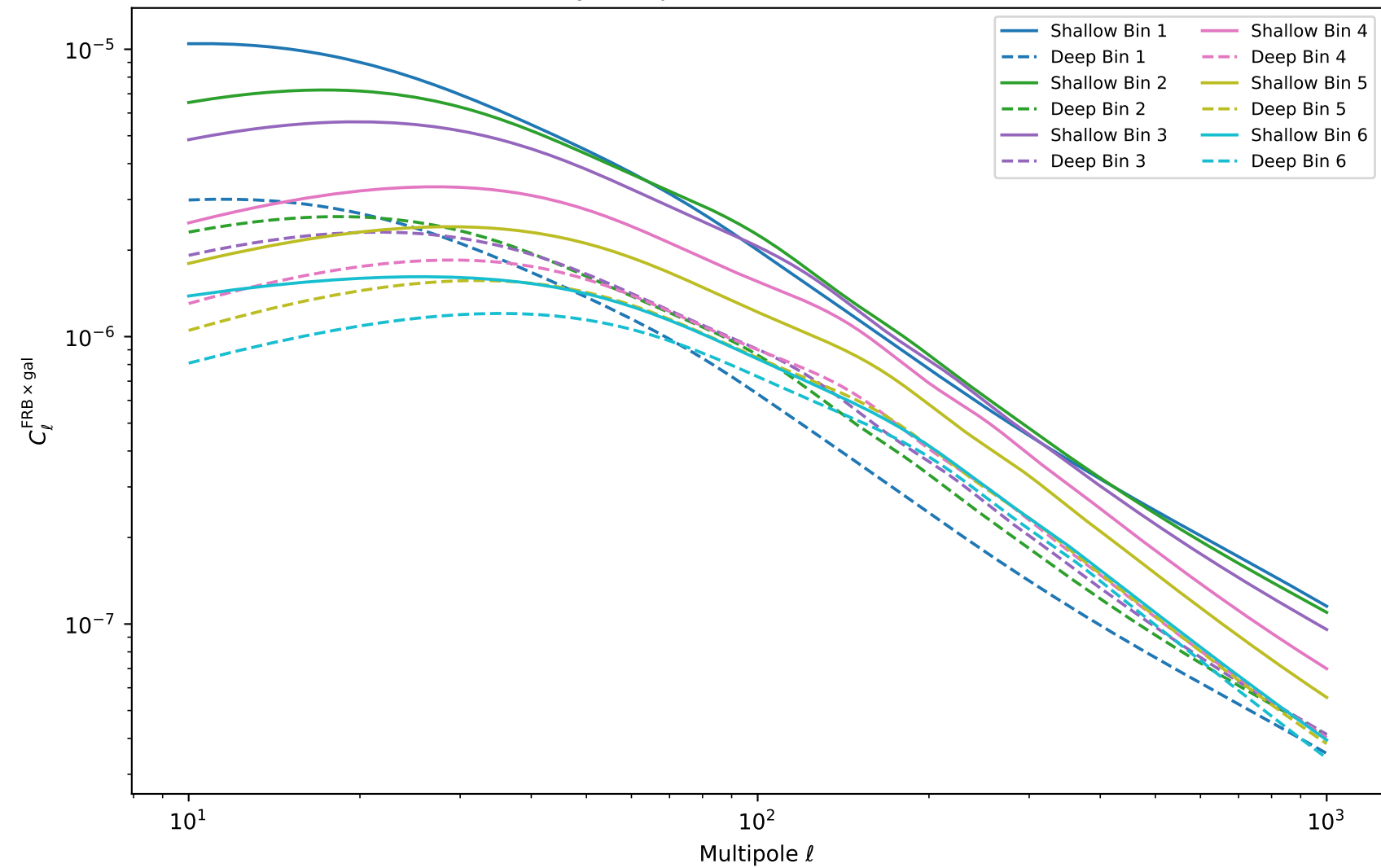
FRB Survey Comparison (Neutron Stars, all bins)
