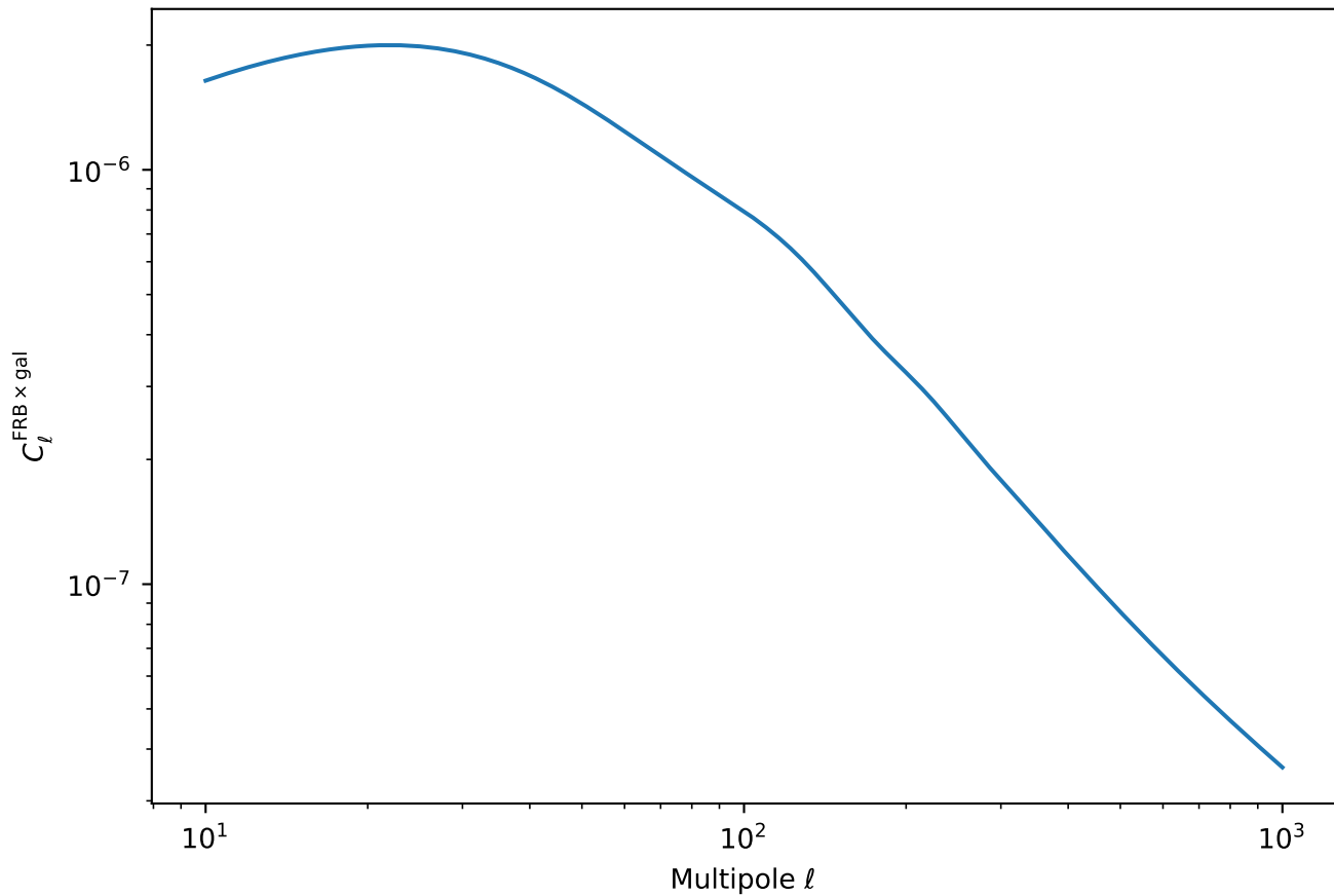
FRB×Galaxy Cross-Correlation (Magnetars, Deep Survey, Galaxy Bin 3)
