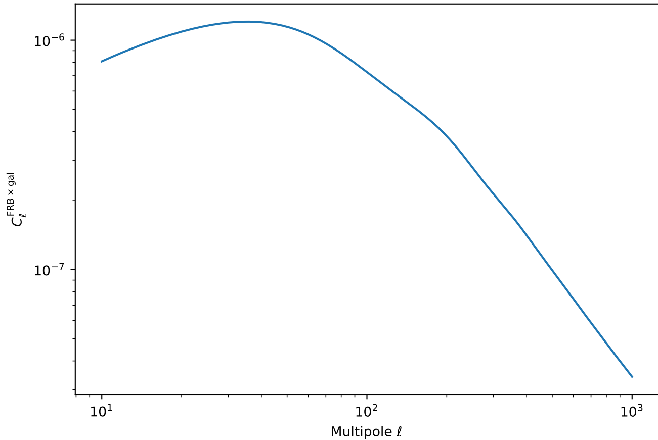
FRB×Galaxy Cross-Correlation (Neutron Stars, Deep Survey, Galaxy Bin 6)
