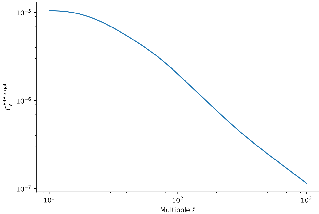
FRB×Galaxy Cross-Correlation (Neutron Stars, Shallow Survey, Galaxy Bin 1)
