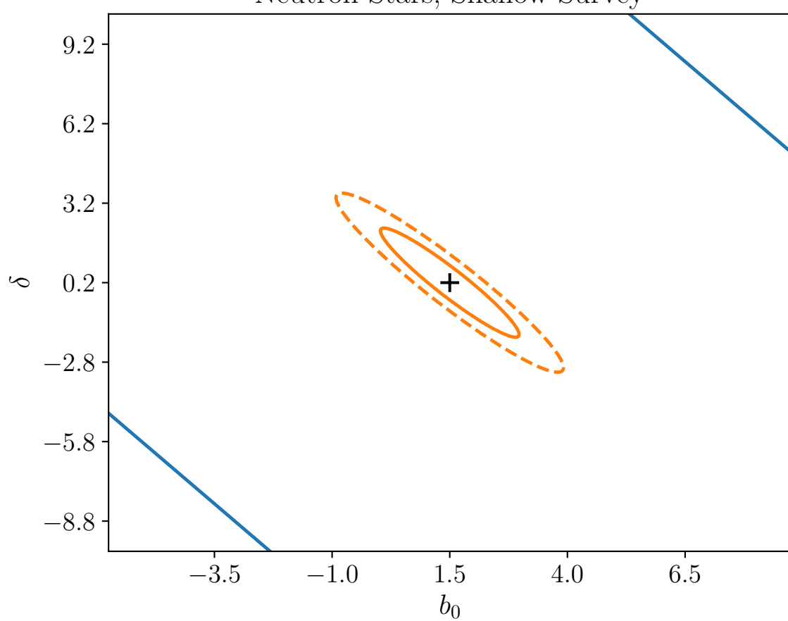
Neutron Stars, Shallow Survey
