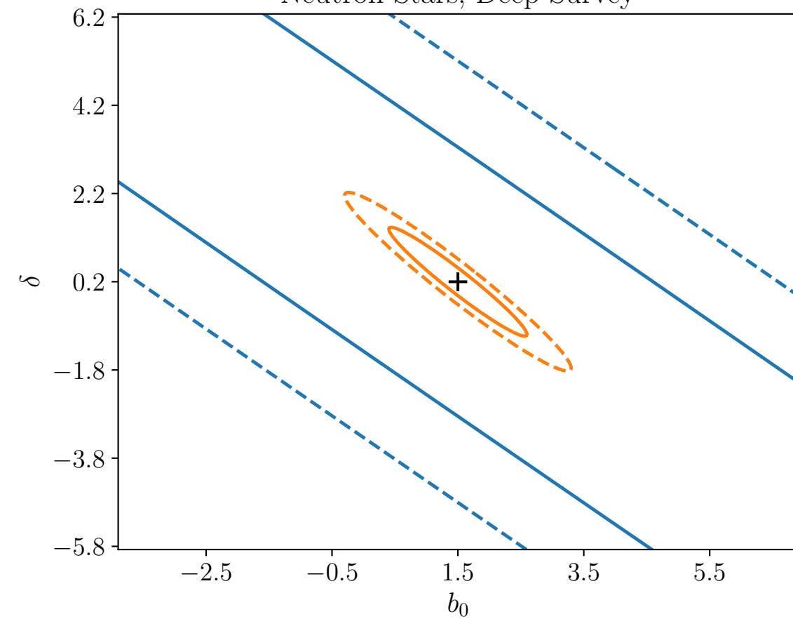
Neutron Stars, Deep Survey
