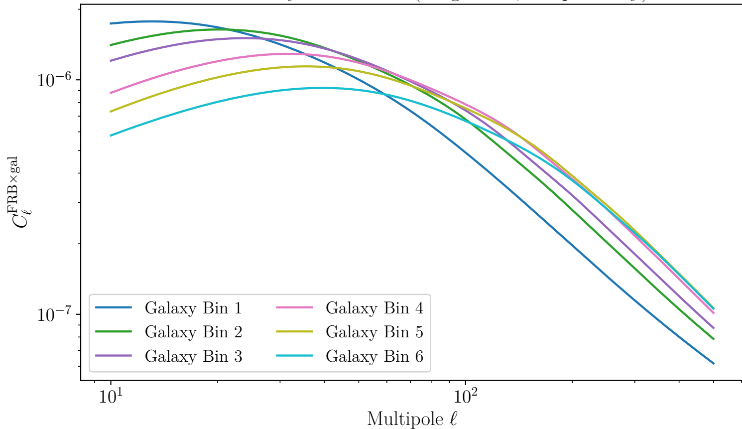
FRB×Galaxy — All Bins (Magnetars, Deep Survey)
