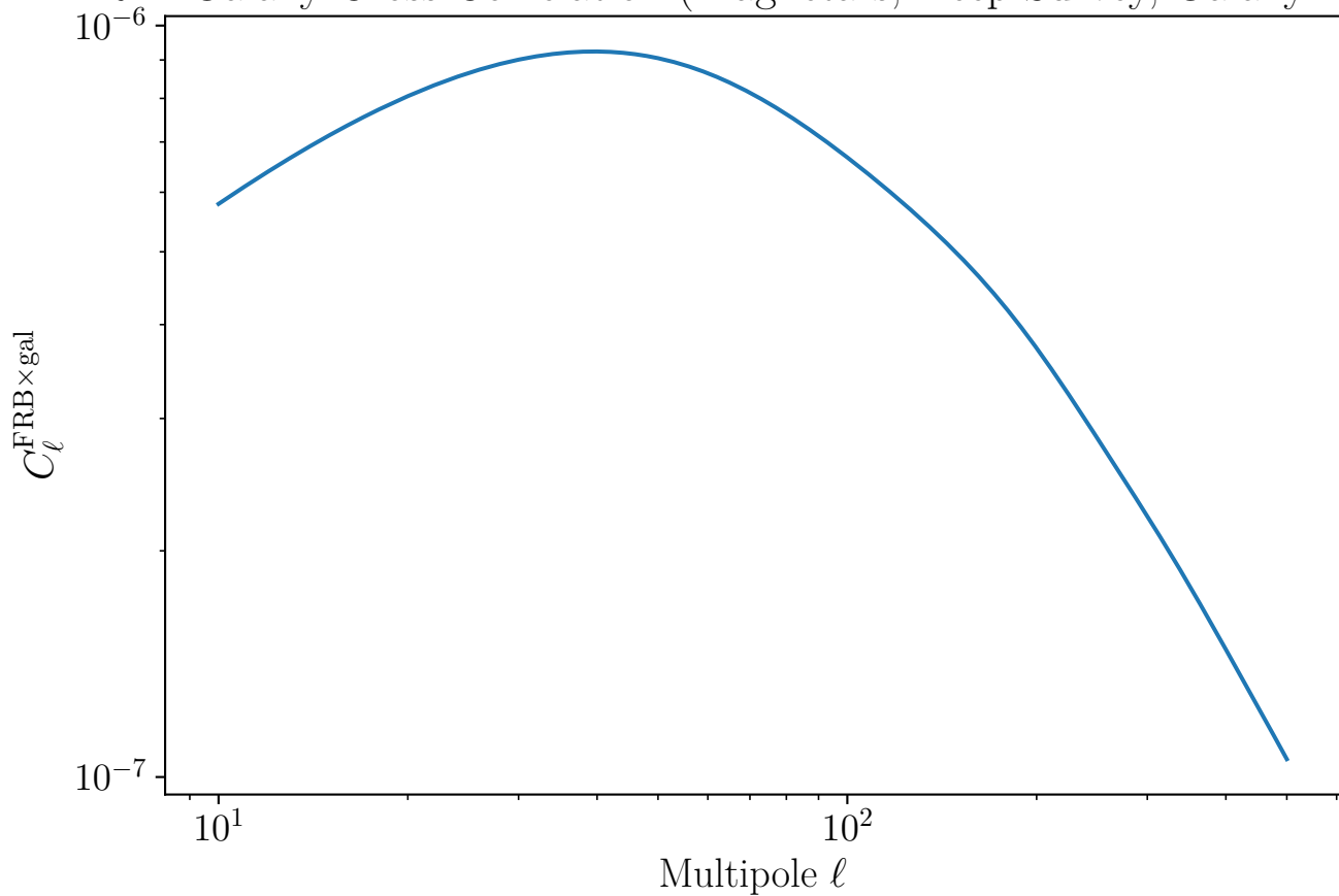
FRB×Galaxy Cross-Correlation (Magnetars, Deep Survey, Galaxy Bin)
