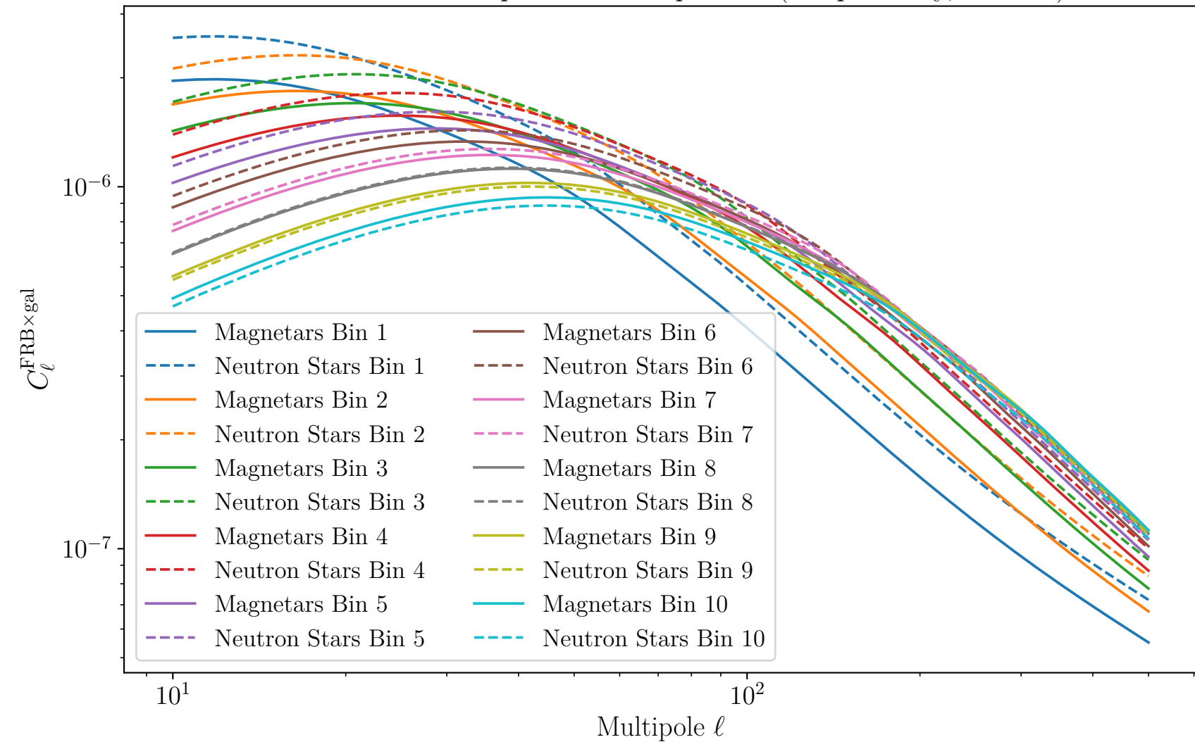
LSST Y10 FRB Population Comparison (Deep Survey, all bins)
