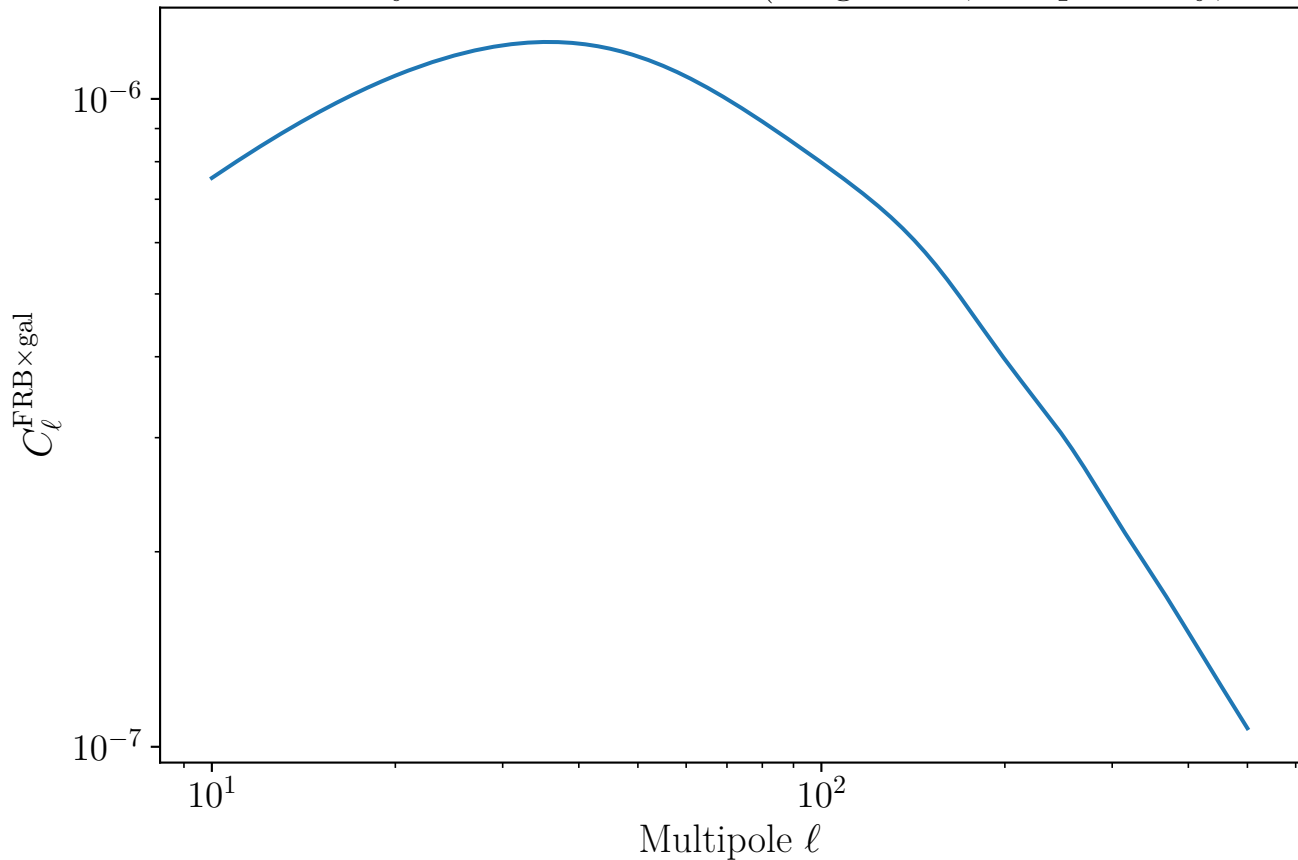
SST Y10 FRB×Galaxy Cross-Correlation (Magnetars, Deep Survey, Galax
