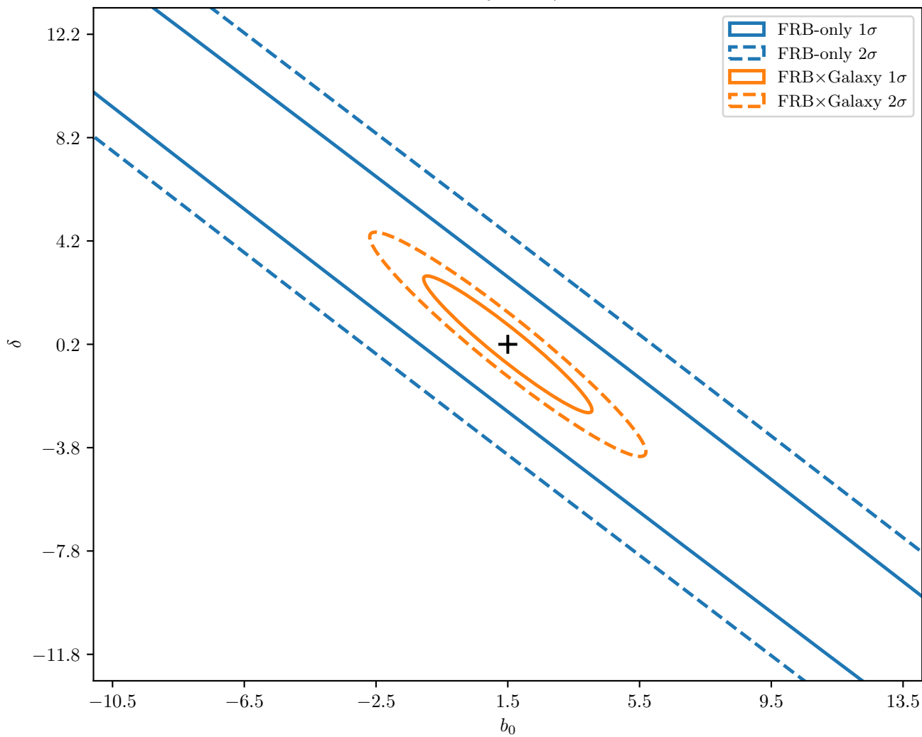
Fisher Forecast — Neutron Stars, Deep Survey Fiducial: b_0 = 1.5 , \delta = 0.2
