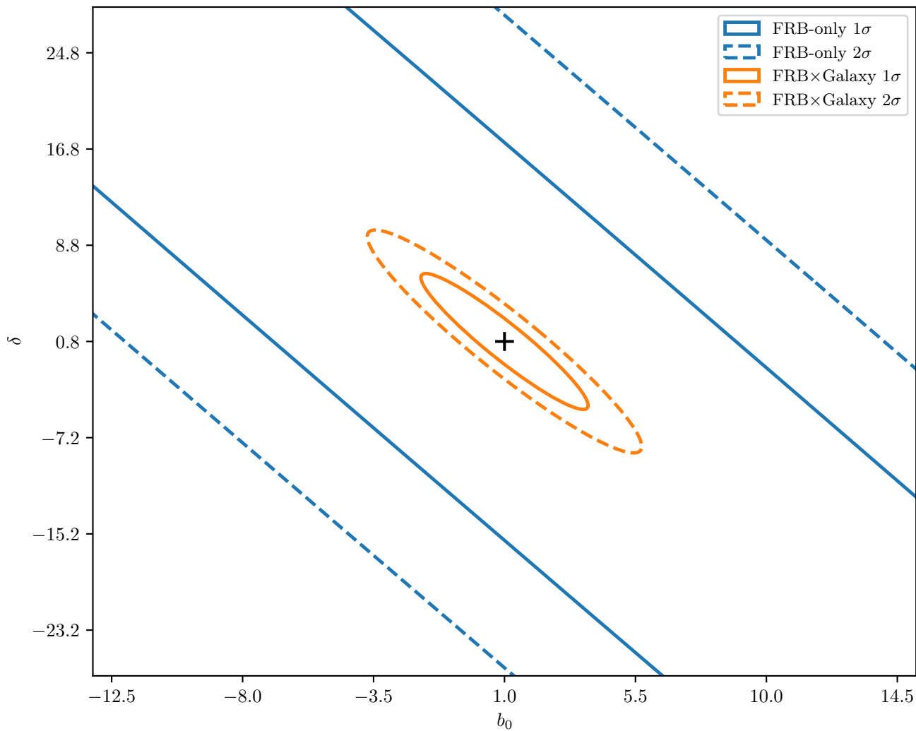
Fisher Forecast — Magnetars, Shallow Survey Fiducial: b_0 = 1.0 , \delta = 0.8
