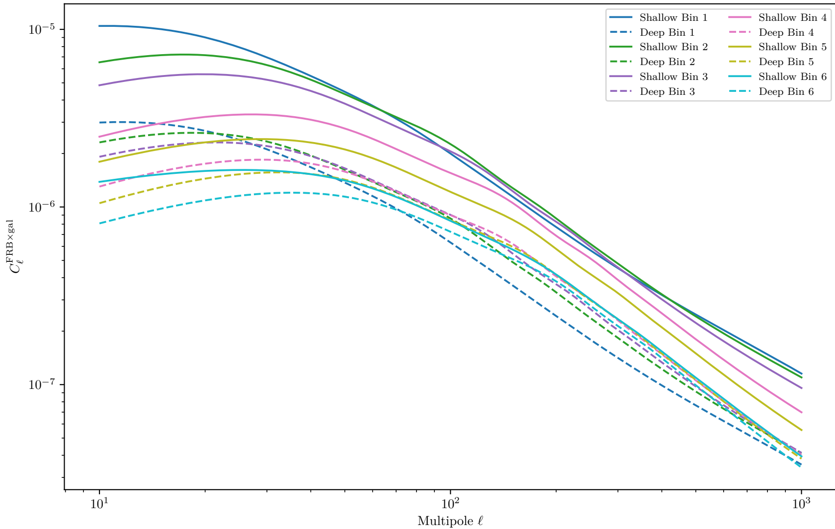
FRB Survey Comparison (Neutron Stars, all bins)
