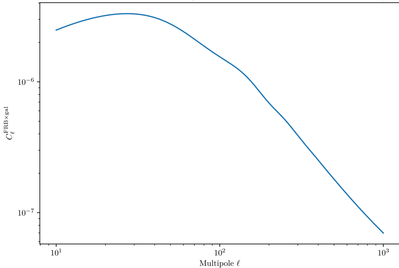
FRB×Galaxy Cross-Correlation (Neutron Stars, Shallow Survey, Galaxy Bin 4)
