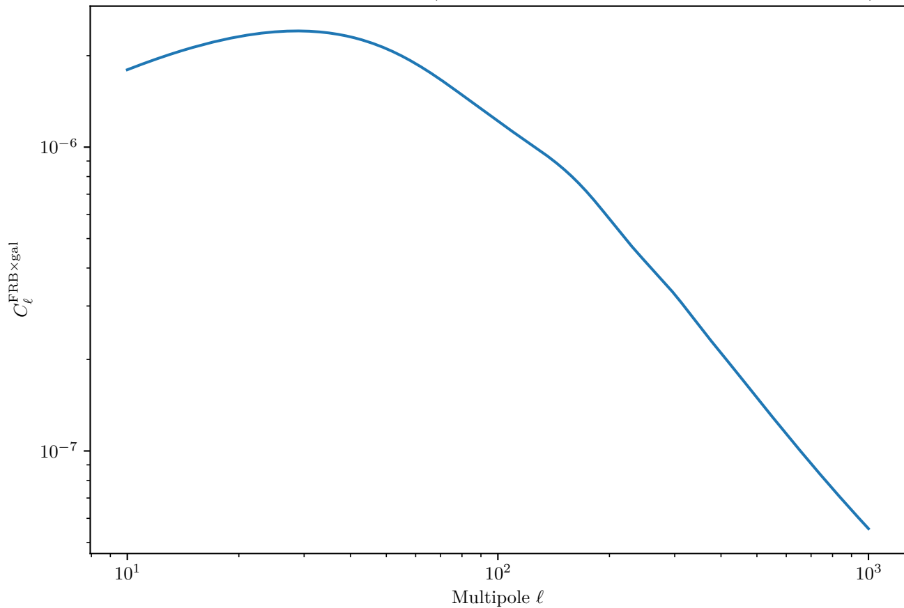
FRB×Galaxy Cross-Correlation (Neutron Stars, Shallow Survey, Galaxy Bin 5)
