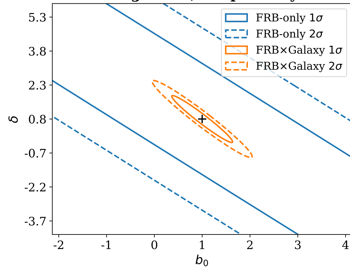
Neutron Stars, Deep Survey
