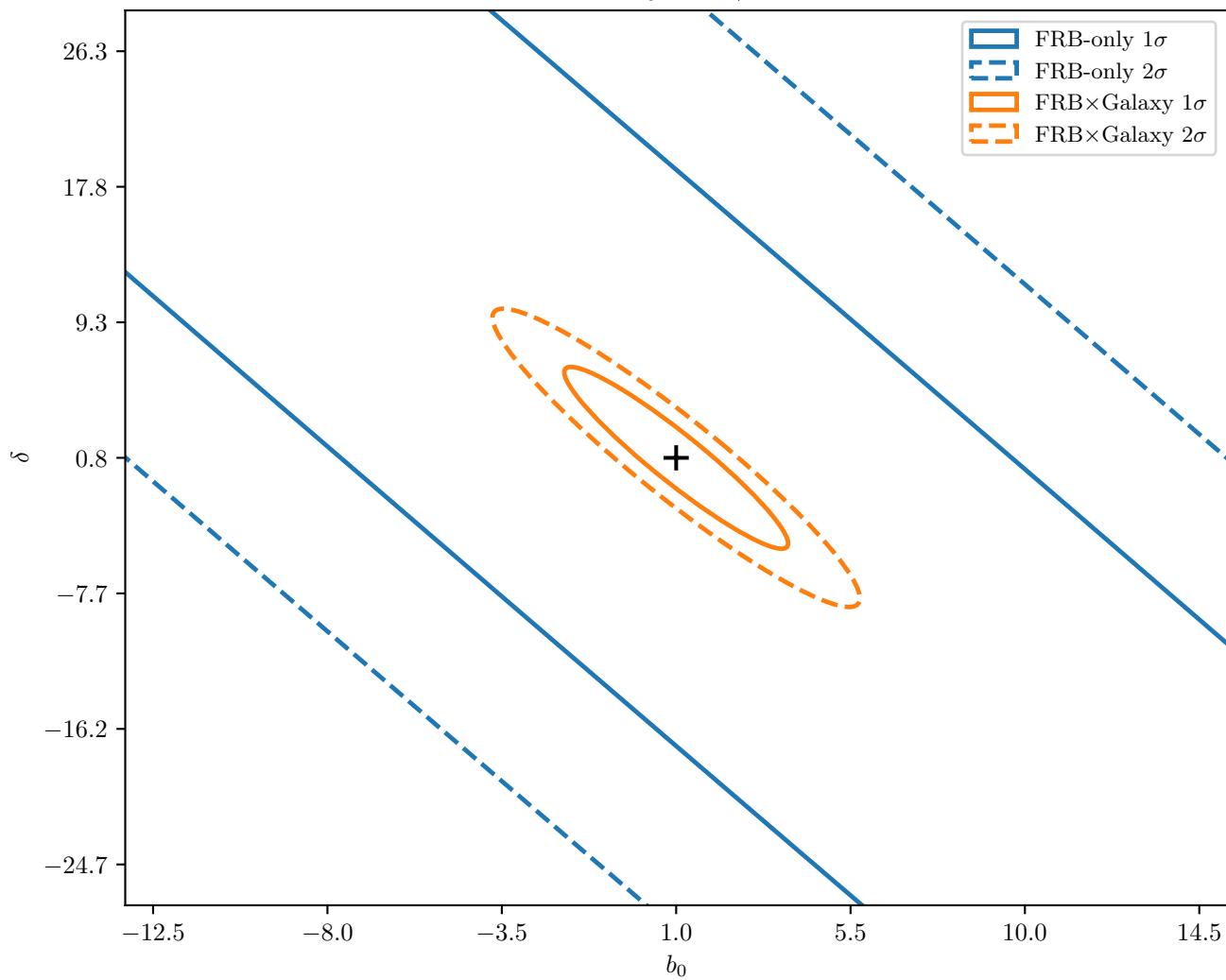
Fisher Forecast — Magnetars, Shallow Survey Fiducial: b_0 = 1.0 , \delta = 0.8
