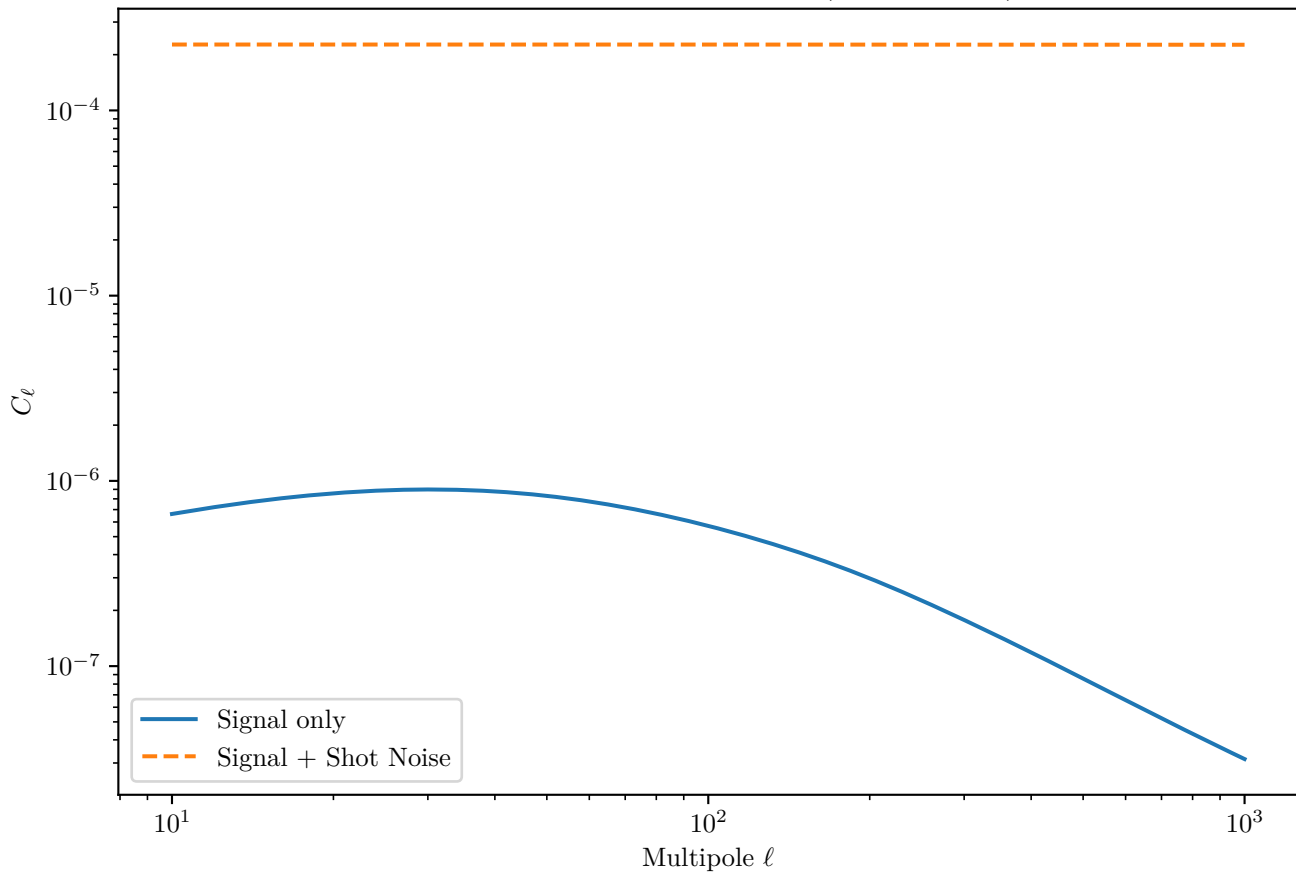
FRB Auto-Correlation Angular Power Spectrum (Deep Survey) for Neutron Stars
