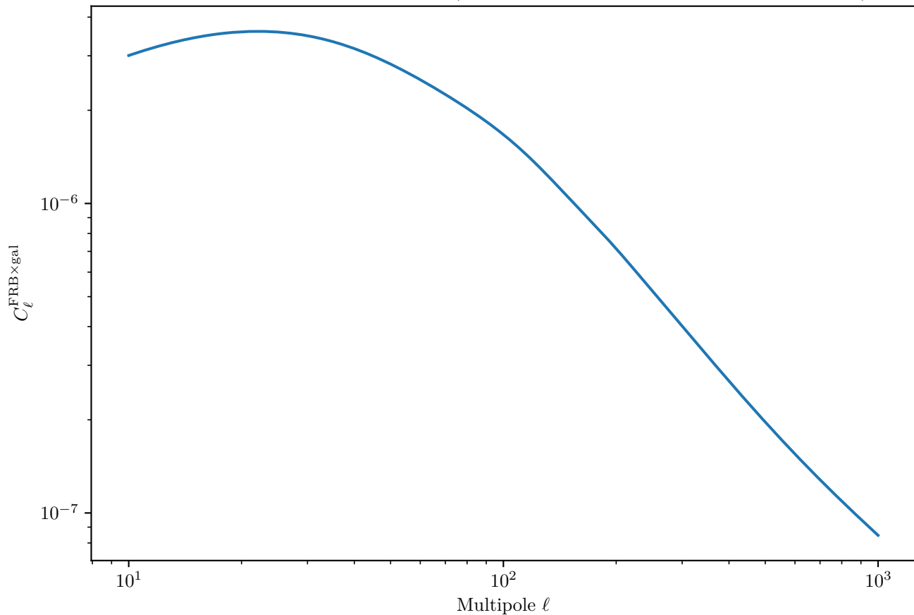
FRB×Galaxy Cross-Correlation (Magnetars, Shallow Survey, Galaxy Bin 3)
