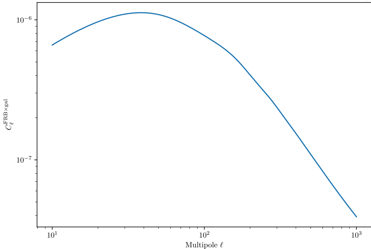
LSST Y10 FRB×Galaxy Cross-Correlation (Magnetars, Deep Survey, Galaxy Bin 6)
