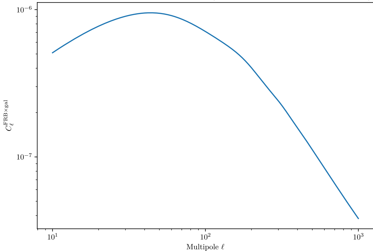
LSST Y10 FRB×Galaxy Cross-Correlation (Magnetars, Deep Survey, Galaxy Bin 7)
