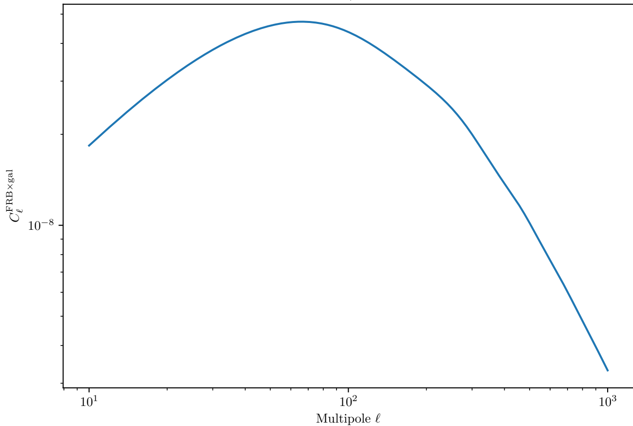
LSST Y10 FRB×Galaxy Cross-Correlation (Magnetars, Shallow Survey, Galaxy Bin 10)
