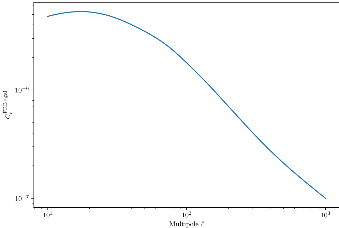
LSST Y10 FRB×Galaxy Cross-Correlation (Magnetars, Shallow Survey, Galaxy Bin 2)
