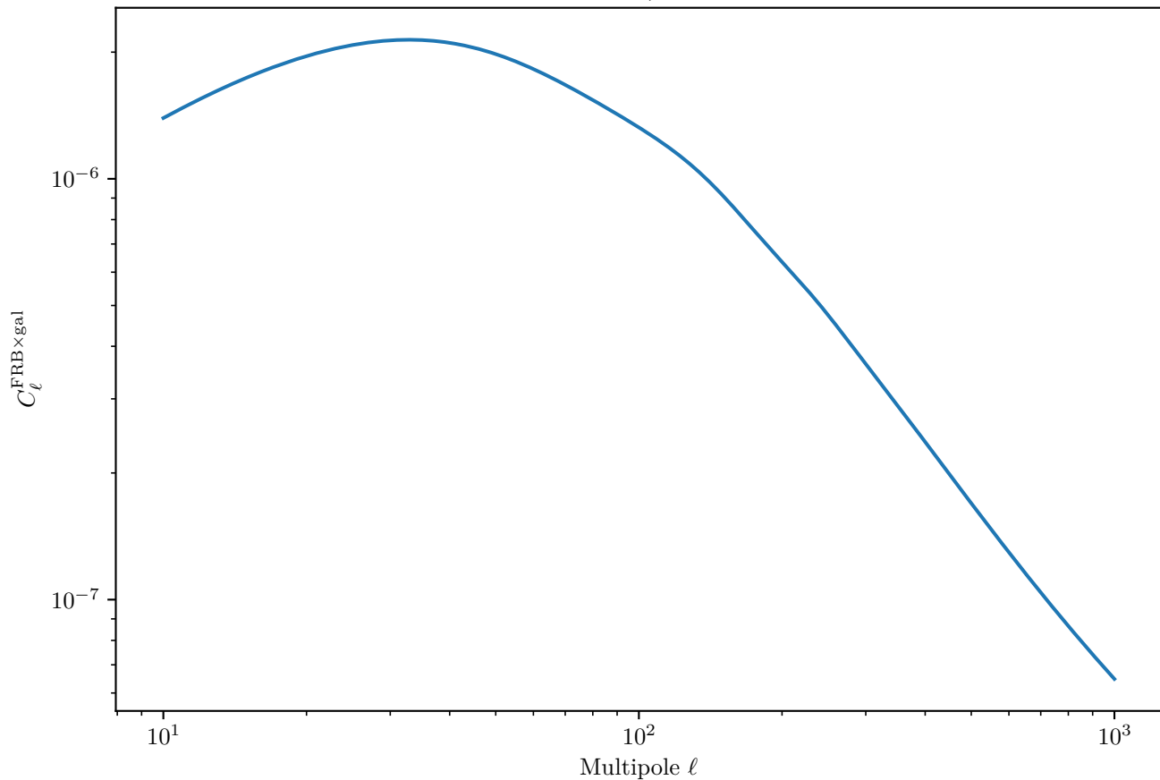
LSST Y10 FRB×Galaxy Cross-Correlation (Magnetars, Shallow Survey, Galaxy Bin 5)
