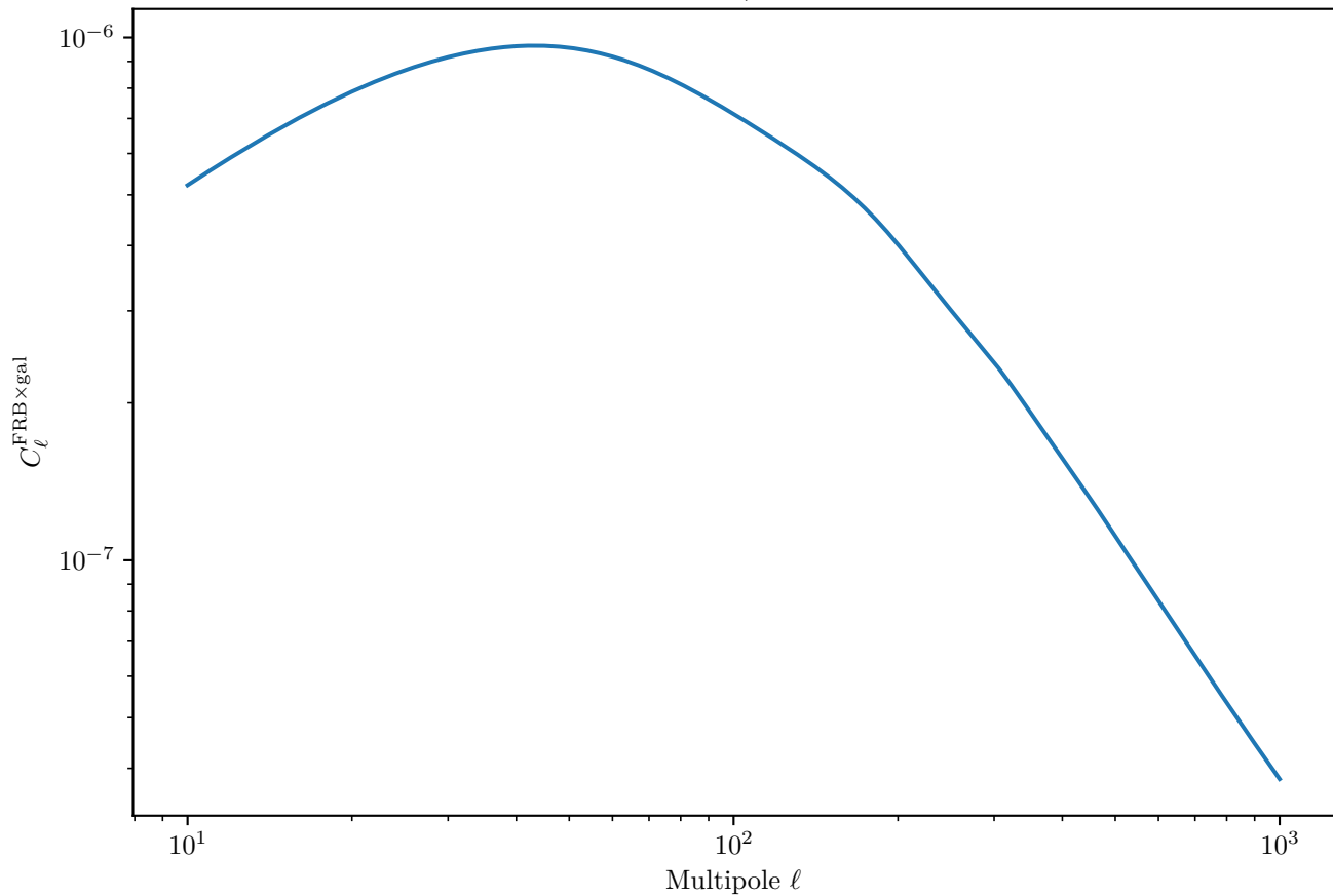
LSST Y10 FRB \times Galaxy Cross-Correlation (Magnetars, Shallow Survey, Galaxy Bin 7)
