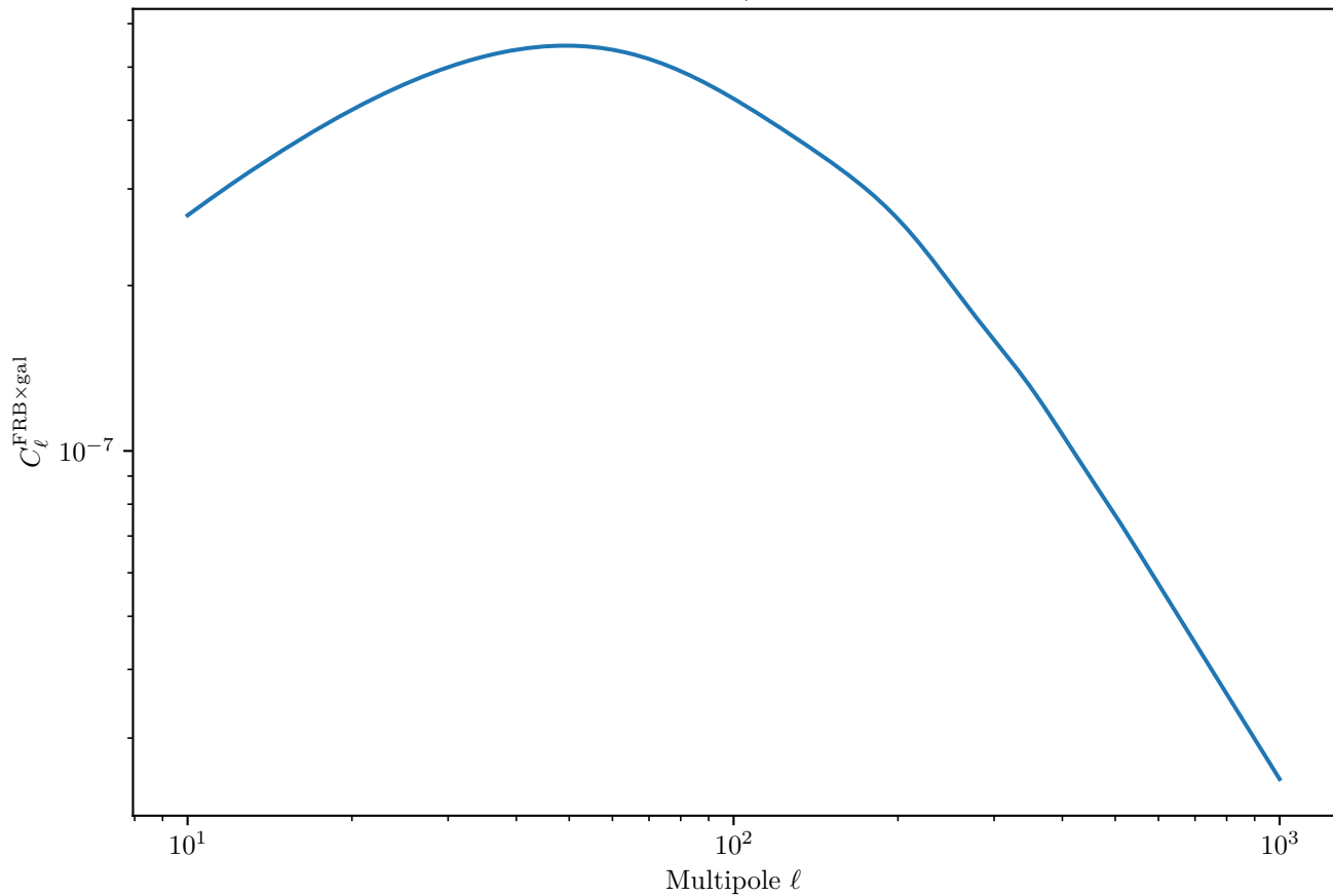
LSST Y10 FRB×Galaxy Cross-Correlation (Magnetars, Shallow Survey, Galaxy Bin 8)
