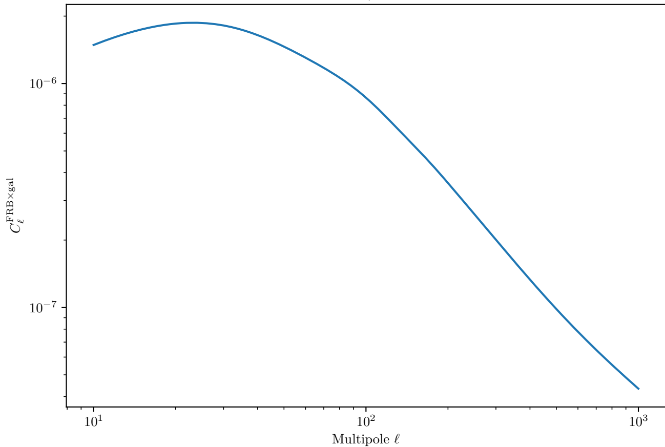
LSST Y10 FRB×Galaxy Cross-Correlation (Neutron Stars, Deep Survey, Galaxy Bin 3)
