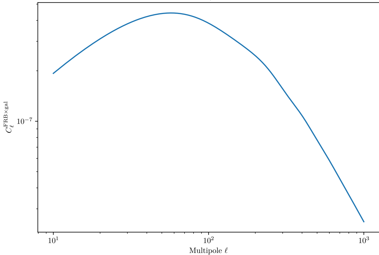
LSST Y10 FRB×Galaxy Cross-Correlation (Neutron Stars, Deep Survey, Galaxy Bin 9)
