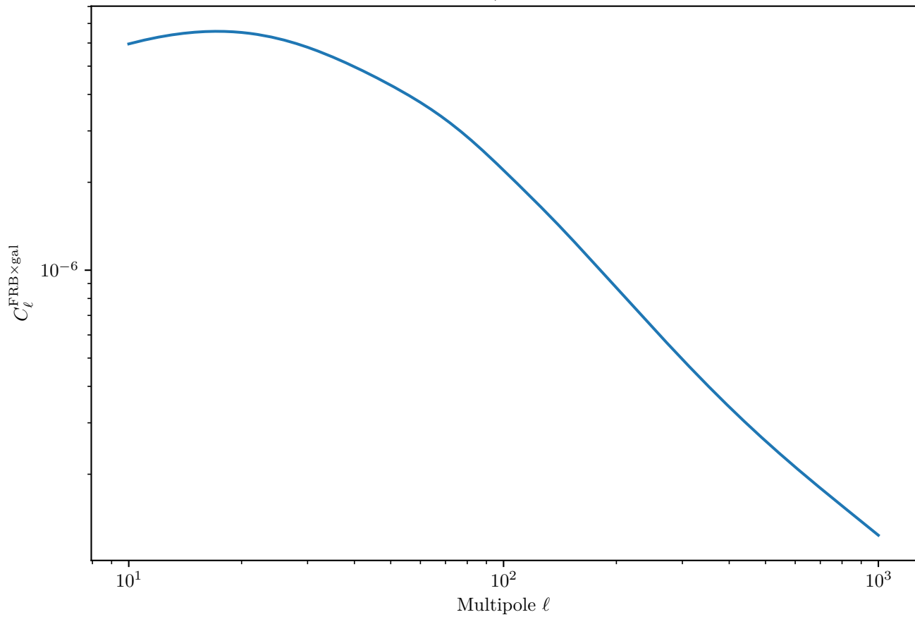
LSST Y10 FRB×Galaxy Cross-Correlation (Neutron Stars, Shallow Survey, Galaxy Bin 2)
