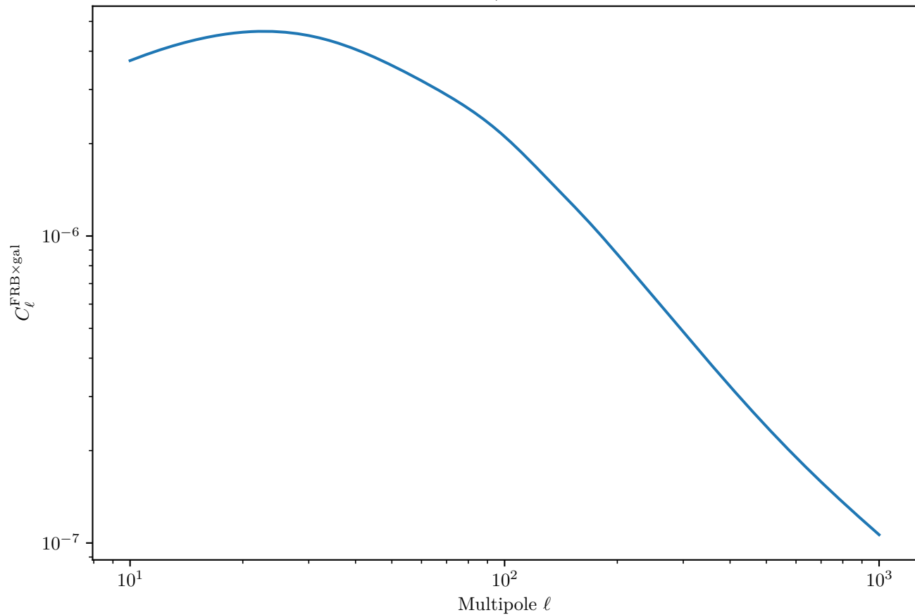
LSST Y10 FRB×Galaxy Cross-Correlation (Neutron Stars, Shallow Survey, Galaxy Bin 3)
