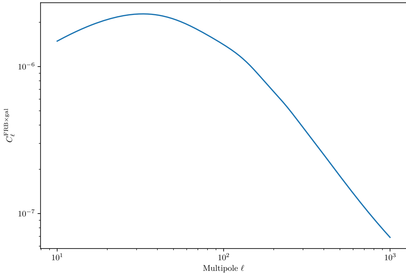
LSST Y10 FRB×Galaxy Cross-Correlation (Neutron Stars, Shallow Survey, Galaxy Bin 5)
