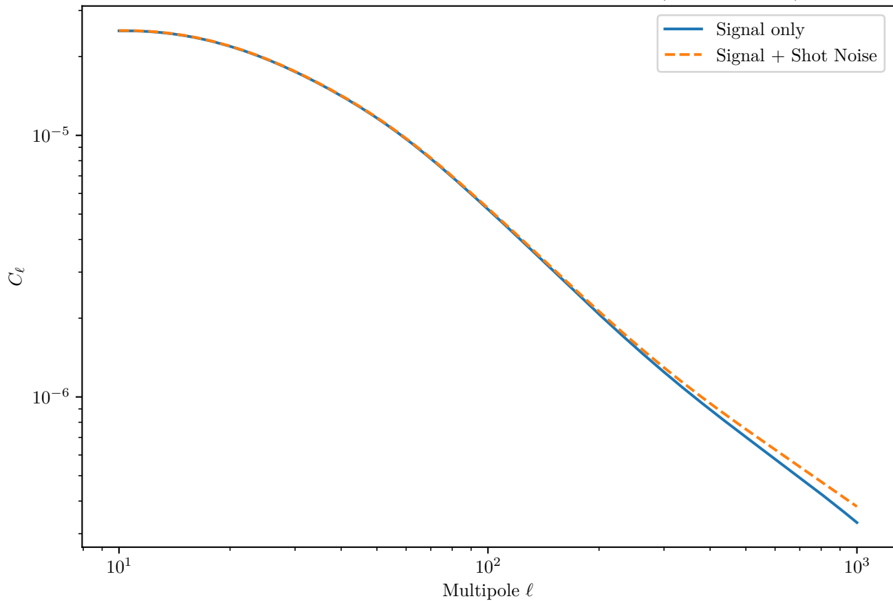
Galaxy Auto-Correlation Angular Power Spectrum (Bin 1 x Bin 1)
