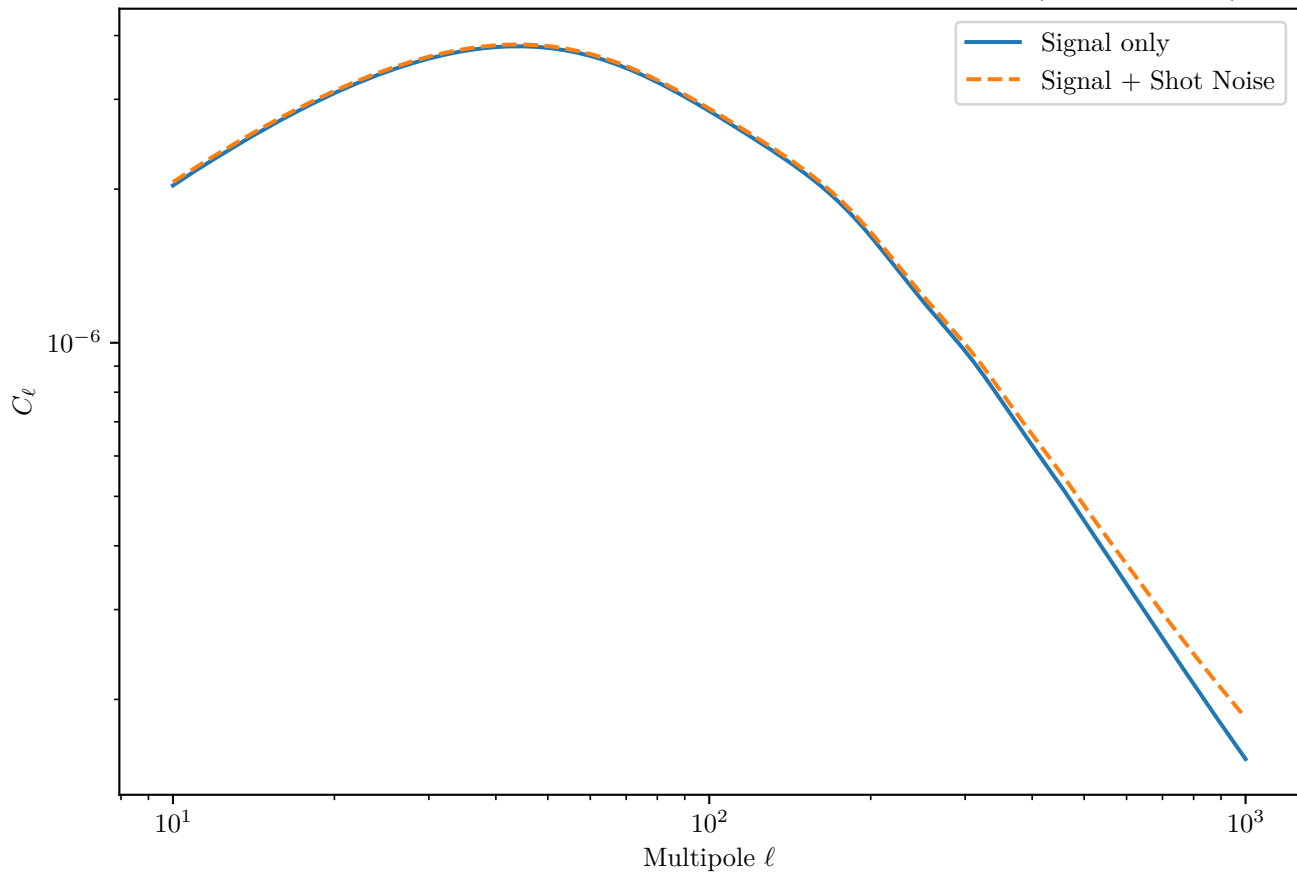
LSST Y10 Galaxy Auto-Correlation Angular Power Spectrum (Bin 7 x Bin 7)
