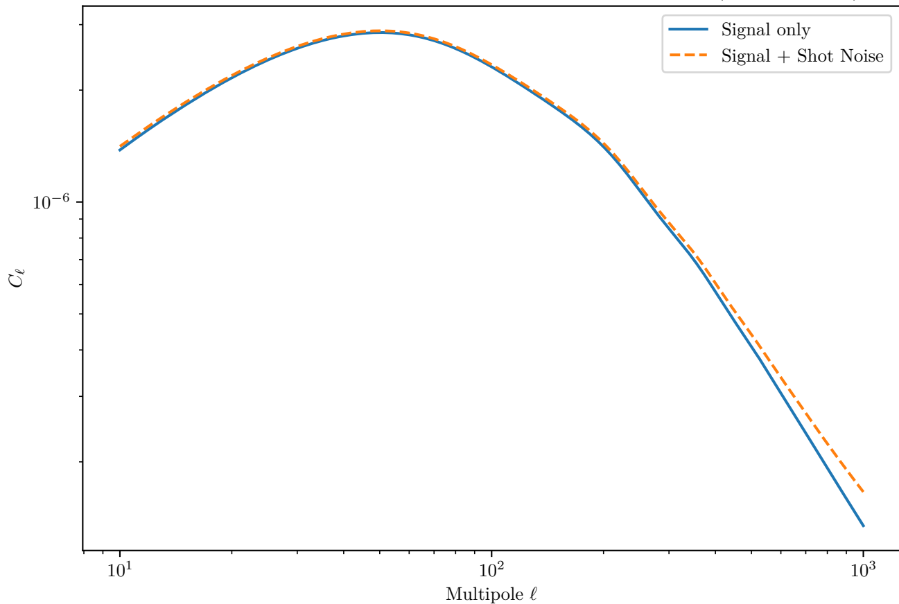
LSST Y10 Galaxy Auto-Correlation Angular Power Spectrum (Bin 8 x Bin 8)
