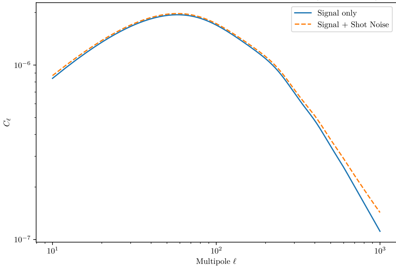
LSST Y10 Galaxy Auto-Correlation Angular Power Spectrum (Bin 9 x Bin 9)
