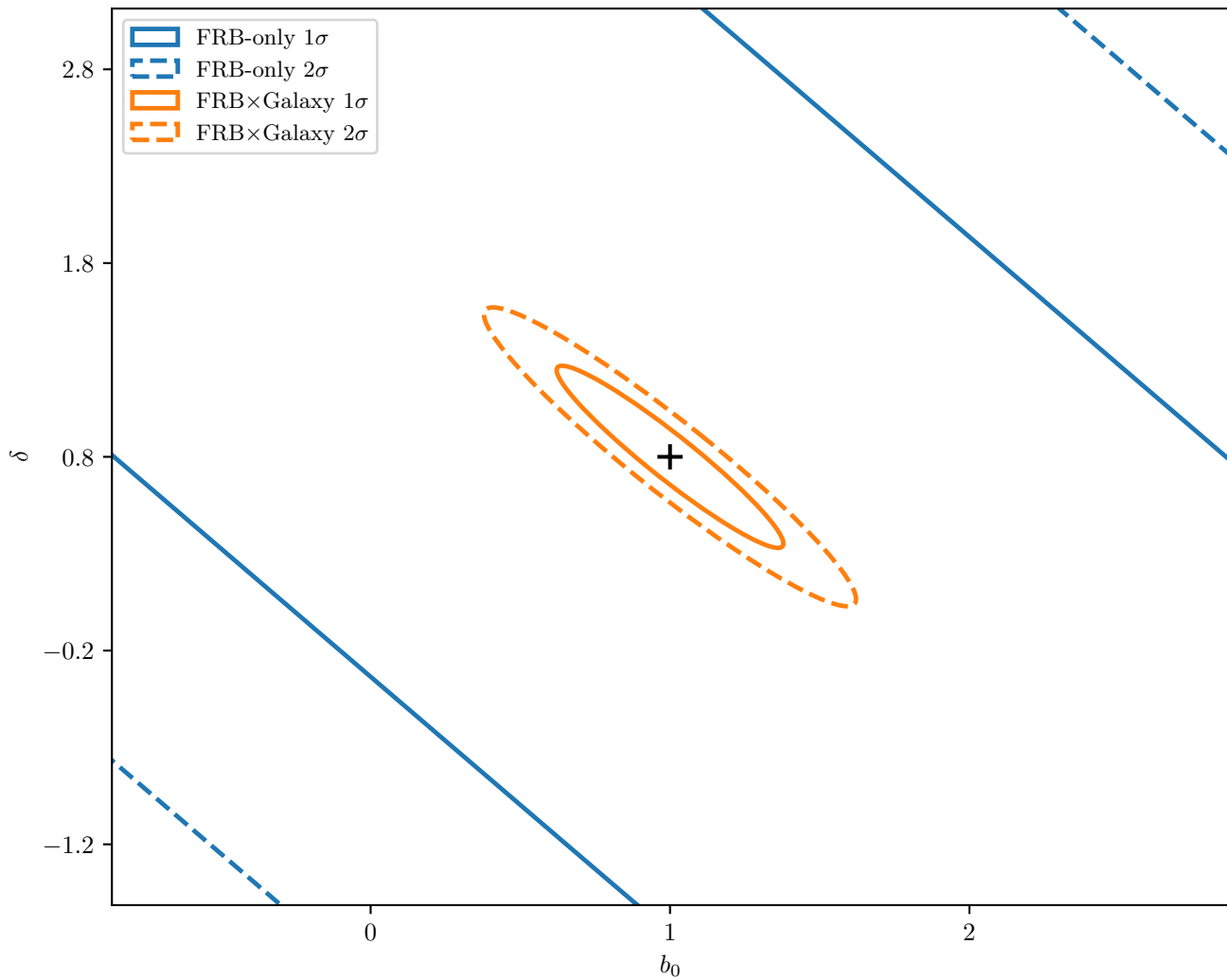
LSST Y10 Fisher Forecast — Magnetars, Deep Survey Fiducial: b_0 = 1.0 , \delta = 0.8
