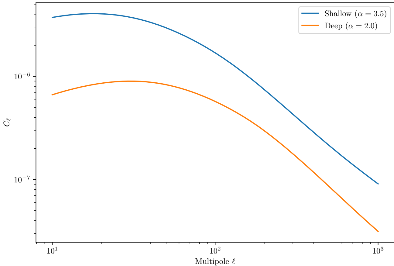
FRB Auto-Correlation: Shallow vs Deep Survey for Neutron Stars
