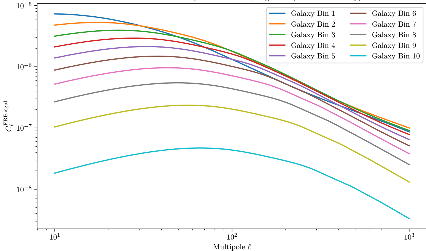
LSST Y10 FRB×Galaxy — All Bins (Magnetars, Shallow Survey)
