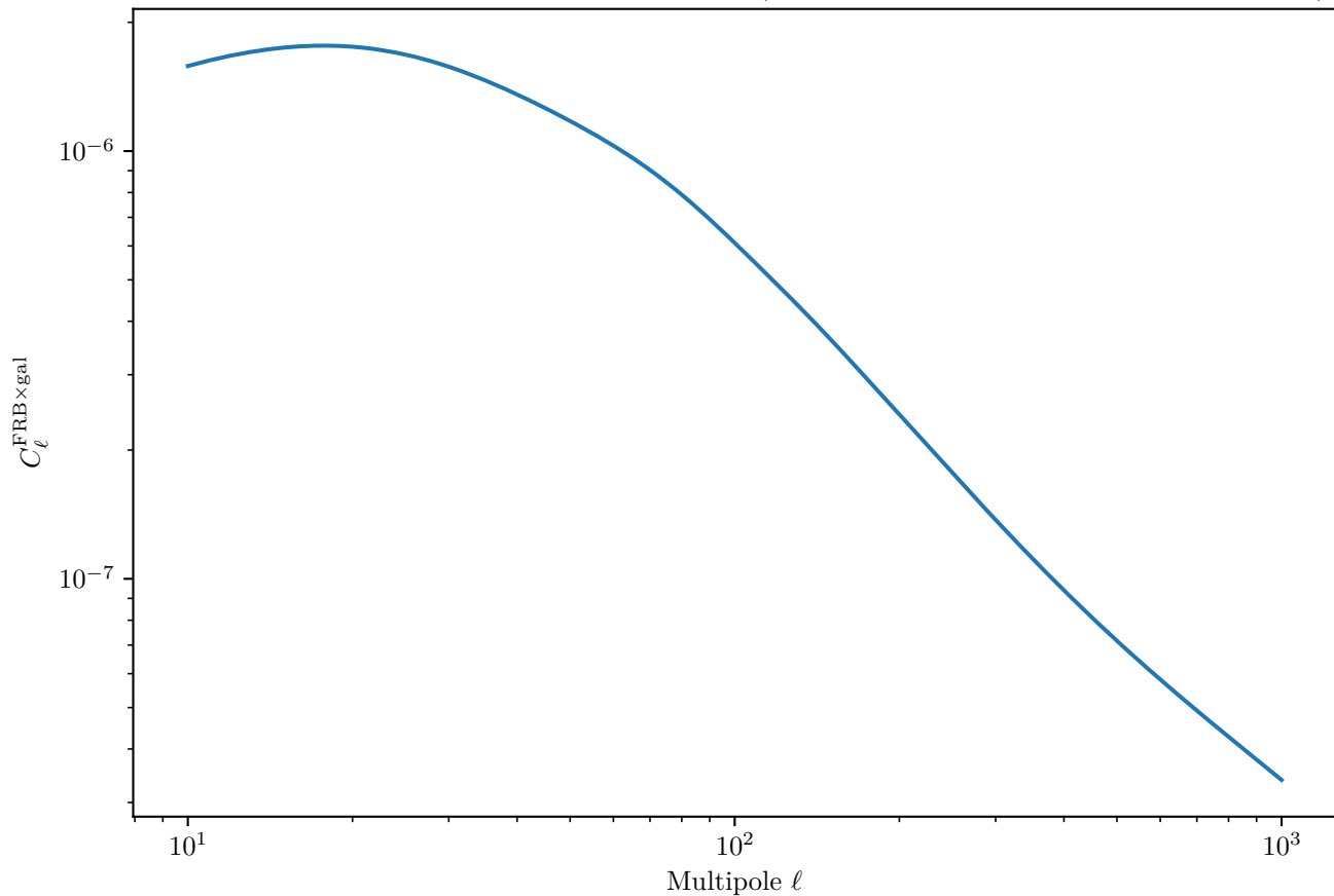
LSST Y10 FRB×Galaxy Cross-Correlation (Magnetars, Deep Survey, Galaxy Bin 2)
