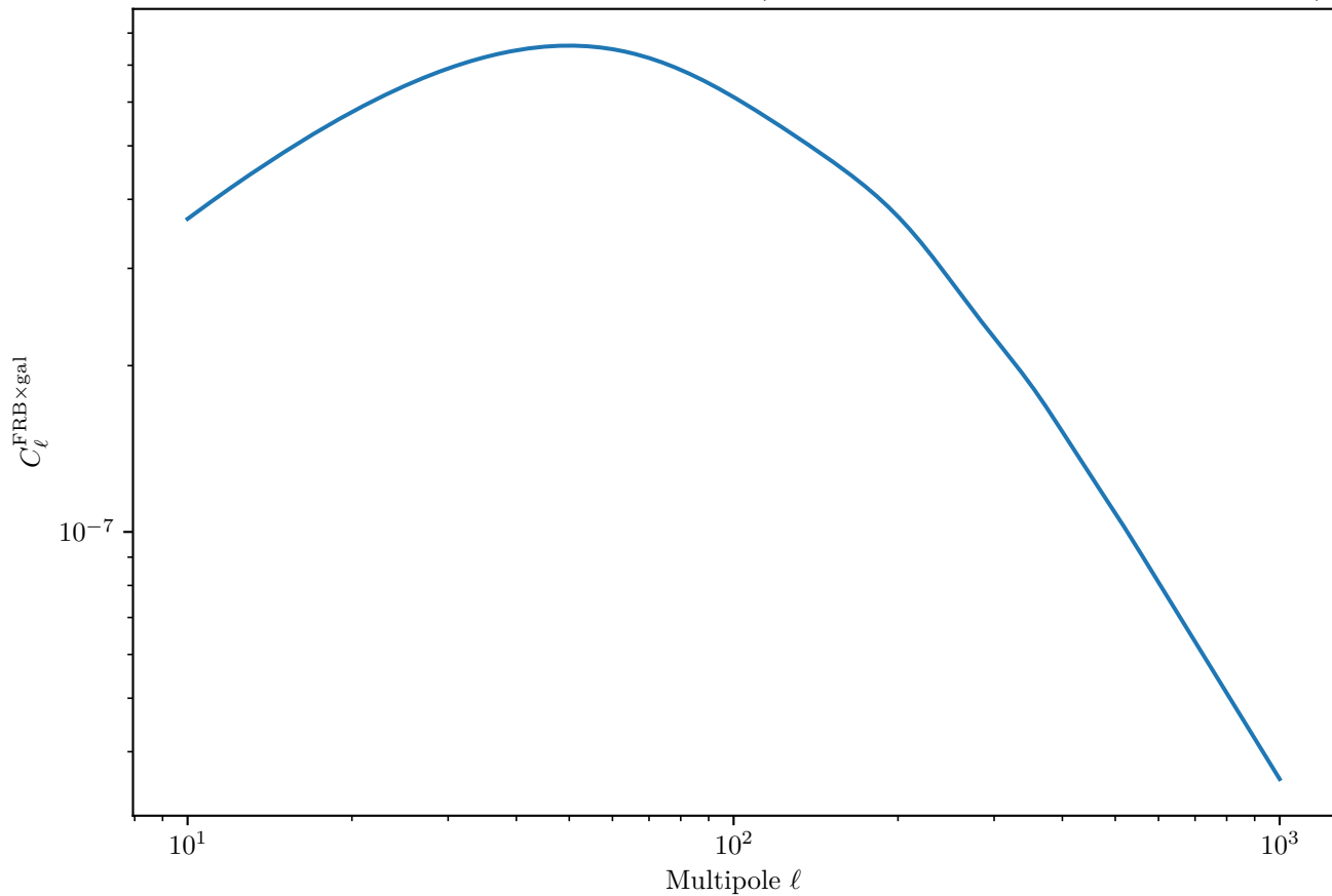
LSST Y10 FRB×Galaxy Cross-Correlation (Magnetars, Deep Survey, Galaxy Bin 8)
