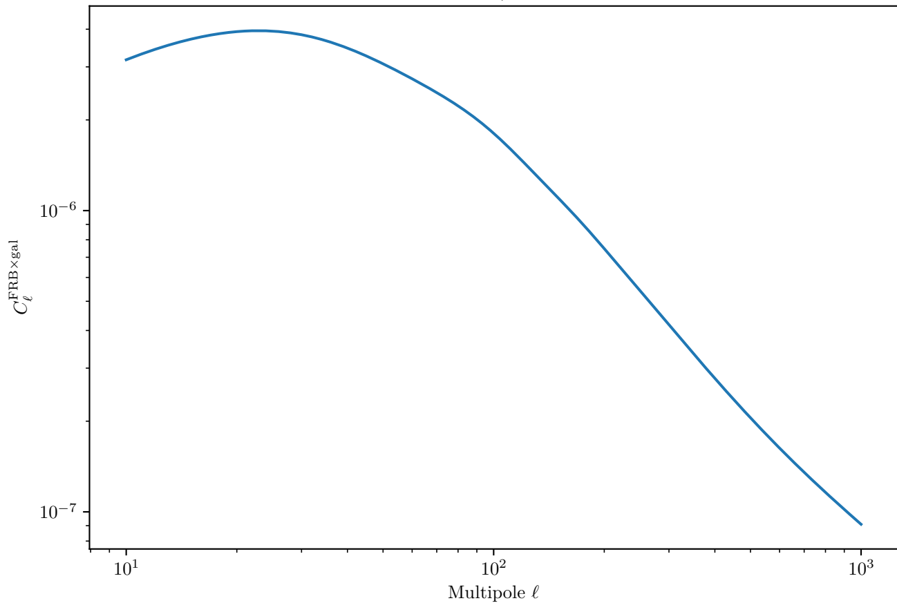
LSST Y10 FRB×Galaxy Cross-Correlation (Magnetars, Shallow Survey, Galaxy Bin 3)
