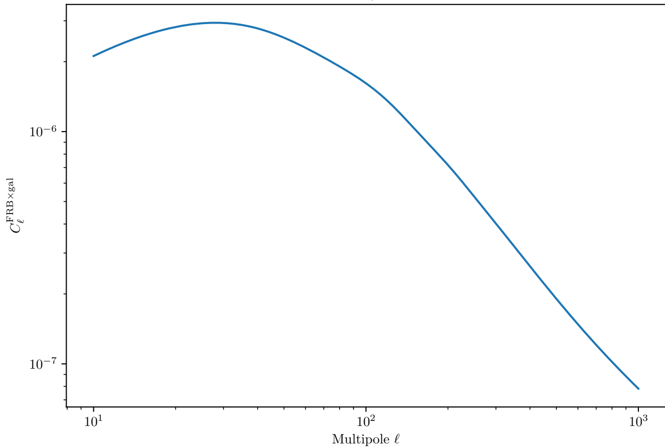
LSST Y10 FRB×Galaxy Cross-Correlation (Magnetars, Shallow Survey, Galaxy Bin 4)
