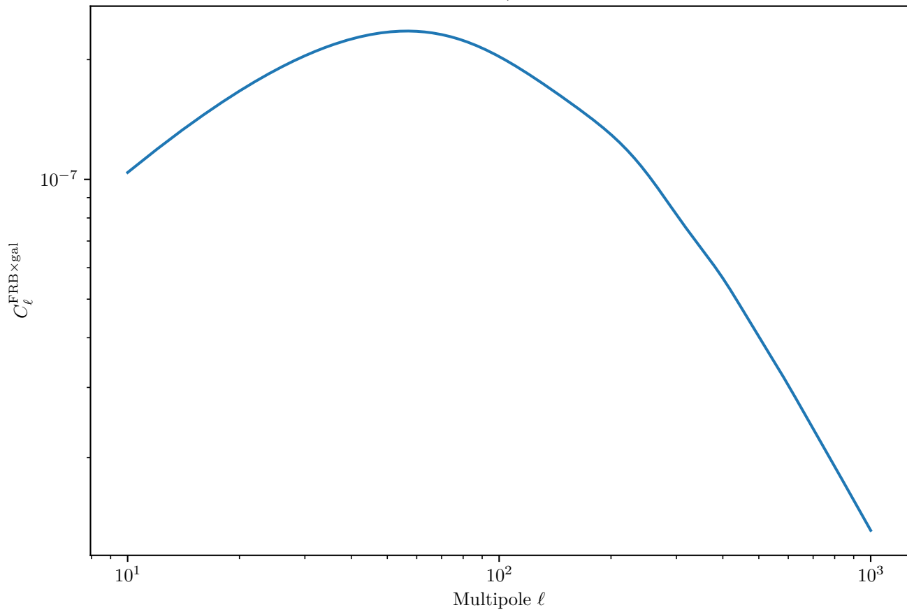
LSST Y10 FRB×Galaxy Cross-Correlation (Magnetars, Shallow Survey, Galaxy Bin 9)
