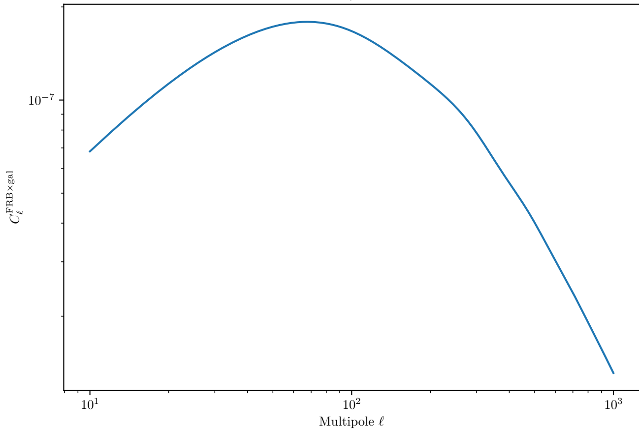
LSST Y10 FRB×Galaxy Cross-Correlation (Neutron Stars, Deep Survey, Galaxy Bin 10)
