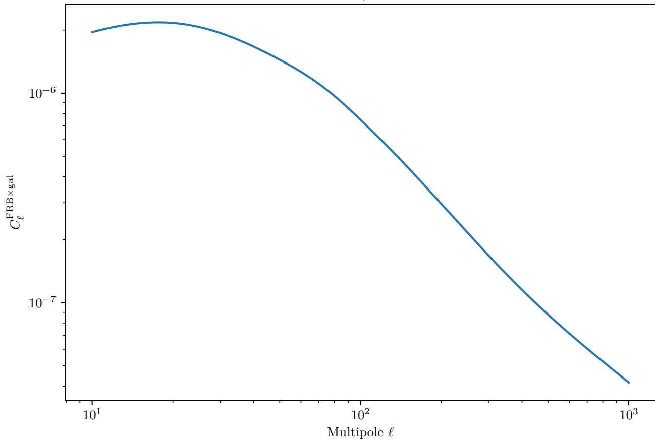
LSST Y10 FRB×Galaxy Cross-Correlation (Neutron Stars, Deep Survey, Galaxy Bin 2)
