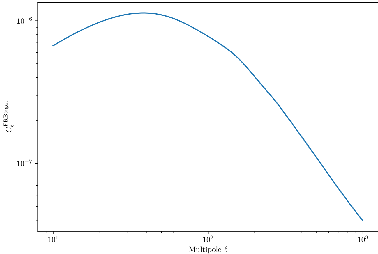
LSST Y10 FRB×Galaxy Cross-Correlation (Neutron Stars, Deep Survey, Galaxy Bin 6)
